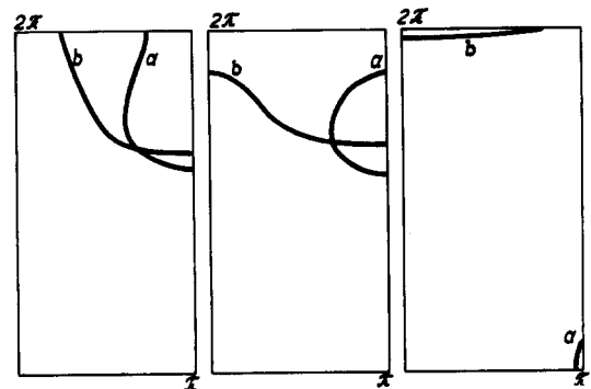
Fig. 1. The curves for parameters a and b , on which the increment is defined, in the fundamental rectangle with the sides \omega = \pi, \omega' = 2\pi . Fig. 1a: |\beta|k = 5 \times 10^{-3} < \wp(\omega + i\omega') - \wp(i\omega') ; fig. 1b: \wp(\omega + i\omega') - \wp(i\omega') < |\beta|k = 0,01 < \wp(\omega) - \wp(\omega + i\omega') ; fig. 1c: \wp(\omega) - \wp(\omega + i\omega') < |\beta|k = 0,25 < \wp(\omega) - \wp(i\omega') .
